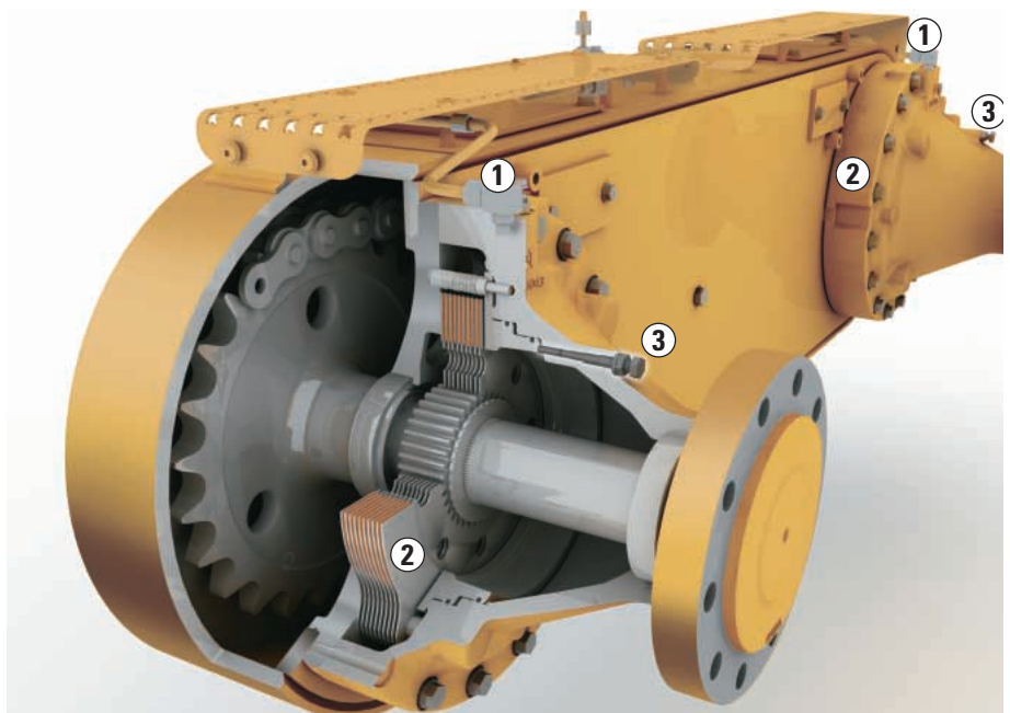
Brake design
